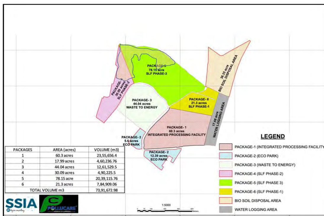
Figure 3: Layout plan of the Six Biomining Packages at KDG
