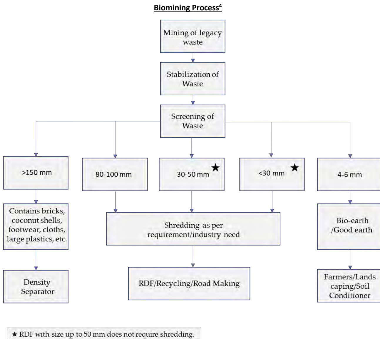
Figure 4: Biomining Process
